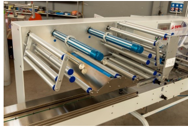
Automatic film reel splicer
