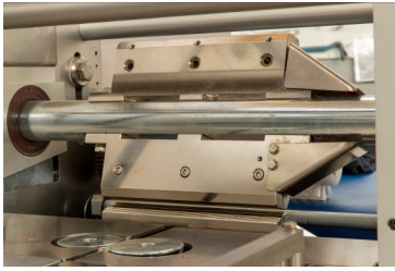
High performance cross sealing head (twin jaws opt)
