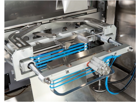
Servo driven sealing jaws with electronically controlled pressure
